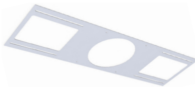
4" Rough-in Plate RP-E4
